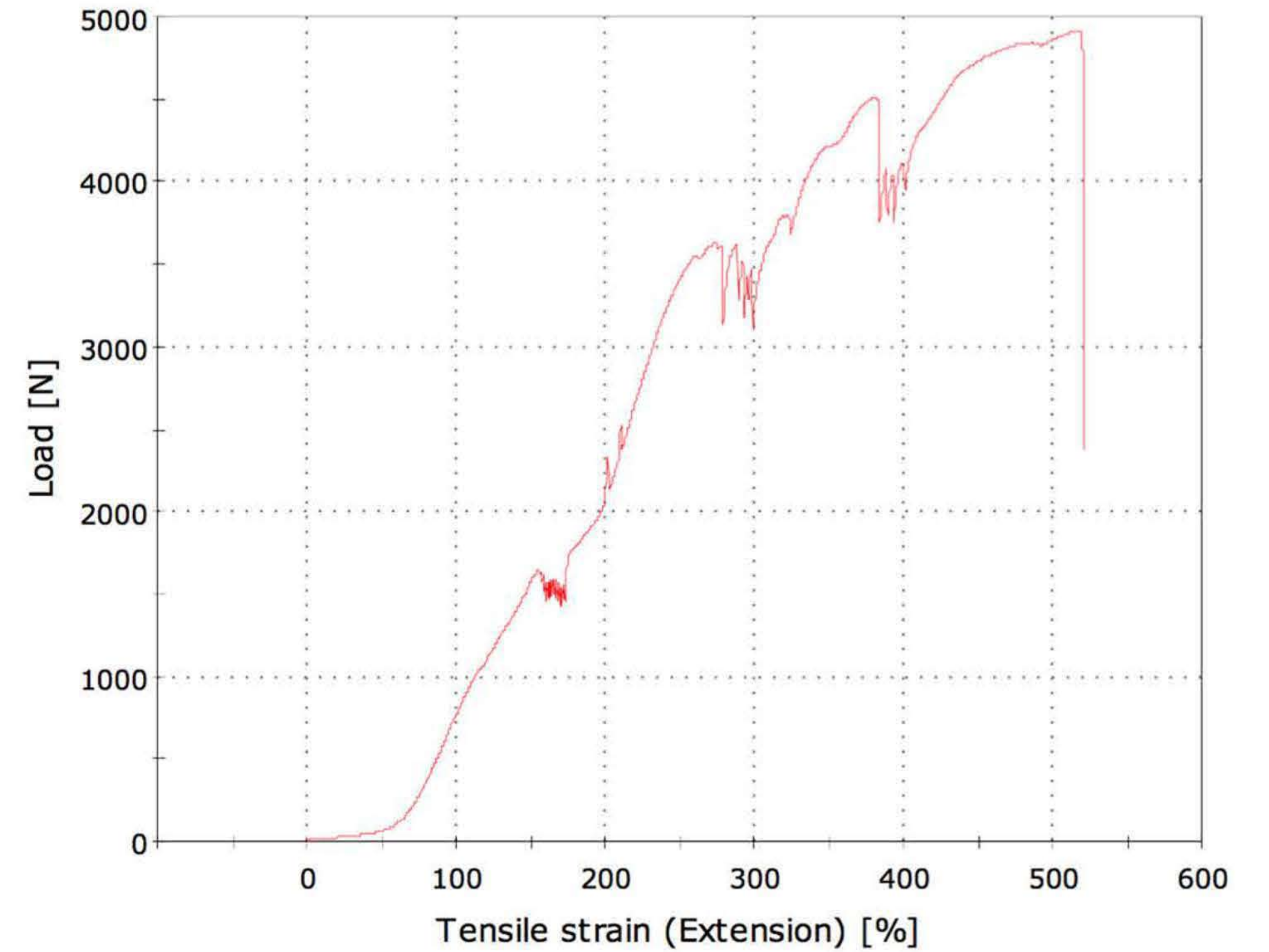
Load-Elongation curve
